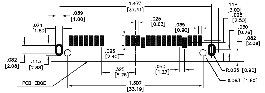
P.C.B. LAYOUT (T=1.2) TOP VIEW
