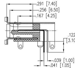
SECT B-B
