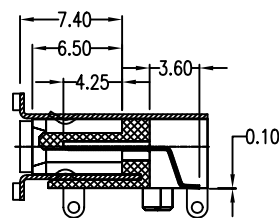
SECT B-B
