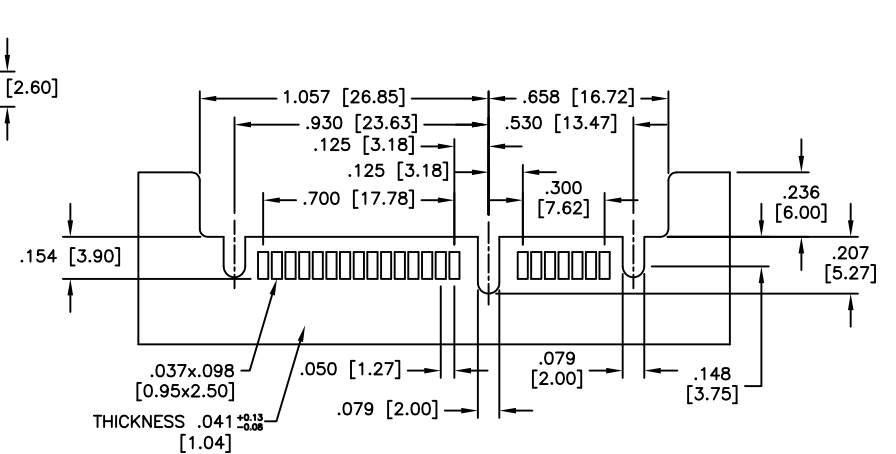
PCB LAYOUT
