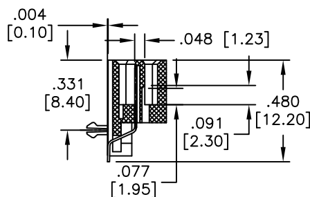
SECT B-B
