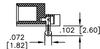
SECT C-C
