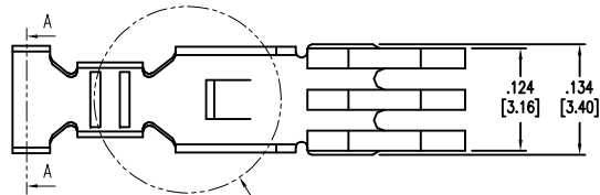
Detail D
