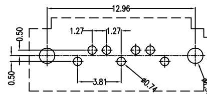
P.C.B. Layout (T=1.60mm)
