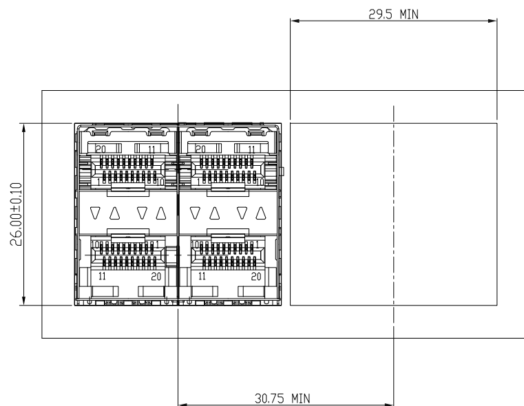
BEZEL CUT-OUT CENTER SPACING DETAIL BEZEL THICKNESS:0.8-2.6
