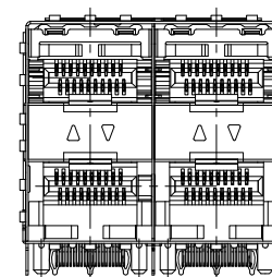
WITH INNER LIGHT PIPES ADAM P/N: SFCJ-4A-LP1
