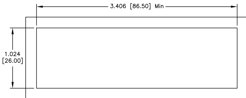
BEZEL CUT-OUT CENTER SPACING DETAIL BEZEL THICKNESS:0.8-2.6
