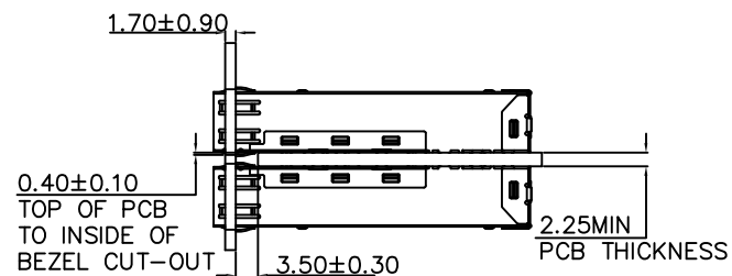
MOUNTED BELLY TO BELLY ON PC BOARD SHOWN TURU RECOMMENDED BEZEL
