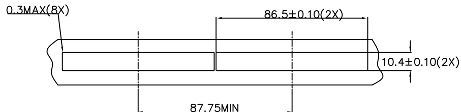
RECOMMENDED BEZEL CUT-OUT SINGLE SIDE APPLICATIONS
