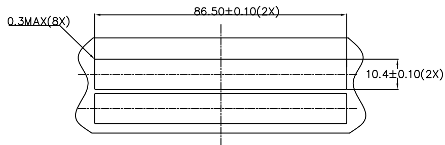
RECOMMENDED BEZEL CUT-OUT BELLY TO BELLY APPLICATIONS
