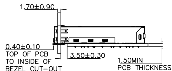
MOUNTED ON PC BOARD SHOWN TURU RECOMMENDED BEZEL
