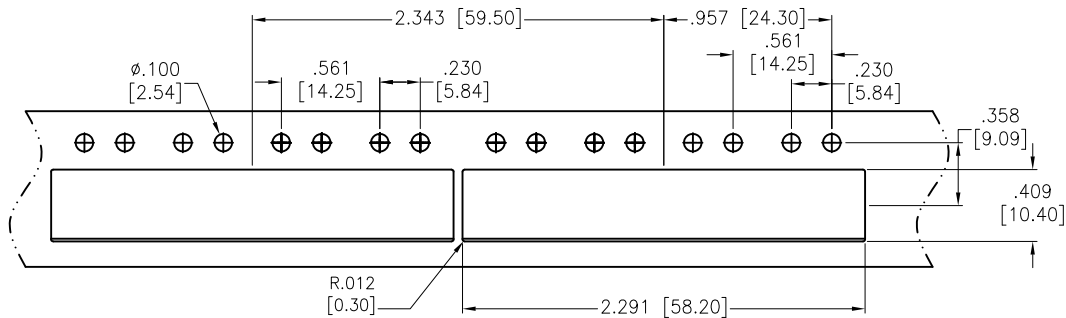
RECOMMENDED BEZEL CUT-OUT SINGLE SIDED APPLICATIONS
