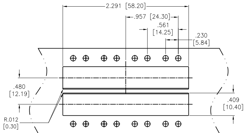
RECOMMENDED BEZEL CUT-OUT BELLY TO BELLY APPLICATIONS
