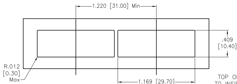
RECOMMENDED BEZEL CUT-OUT SINGLE SIDED APPLICATIONS
