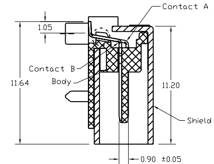
SECT:A-A
