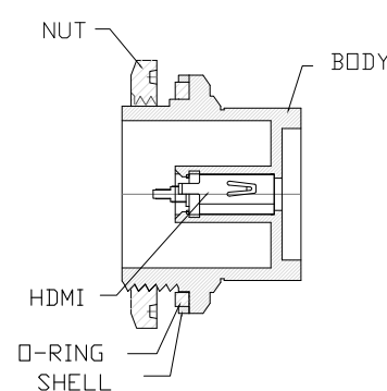
Assembly SECTION A-A
