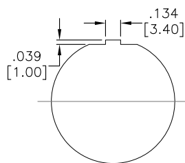
PANEL CUT-OUT
