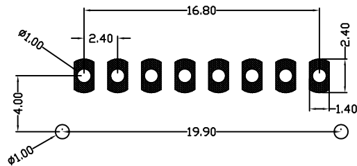
PCB LAYOUT Layout Tolerance: \pm 0.05\text{mm}
