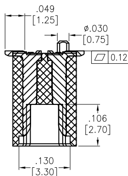
SECTION E-E
