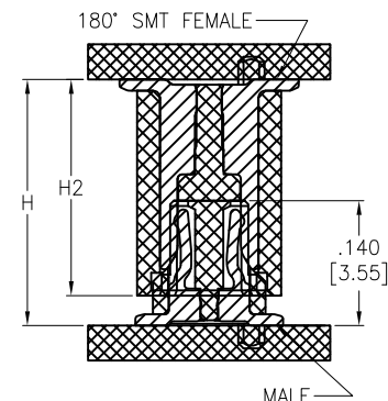
ASSEMBLY VIEW
