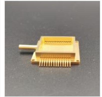
Hermetically Sealed Packages
