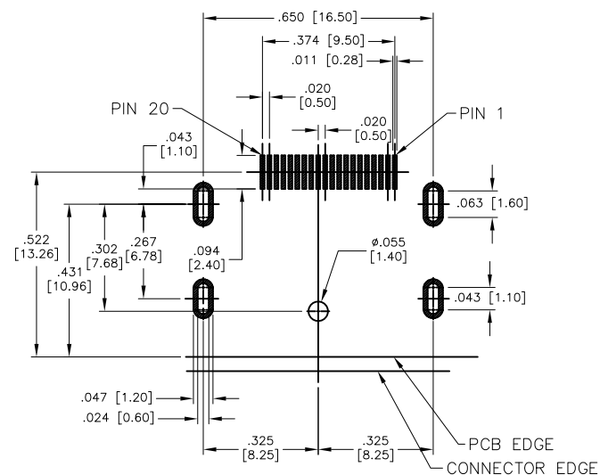
RECOMMENDER PCB LAYOUT(THICKNESS=1.6±0.15)
