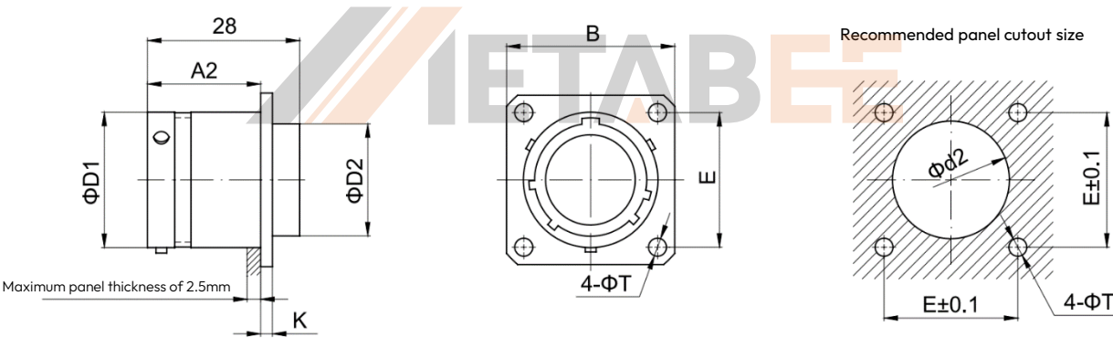
Rear Mount Box-Type Flange Receptacle MS27505
