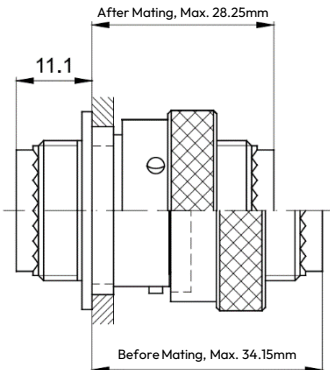
MS27497 Receptacle / MS27473 Plug
