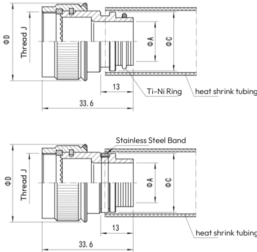
M85049/88 Straight
