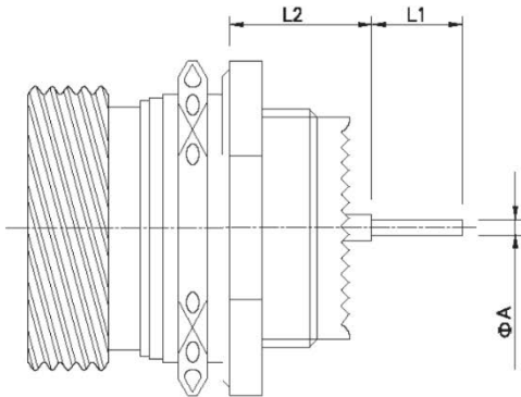
D38999/24 Receptacle
