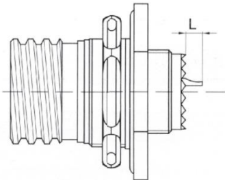
D38999/26 Receptacle
