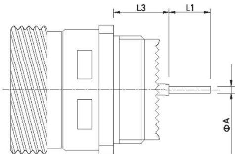
D38999/20 Receptacle
