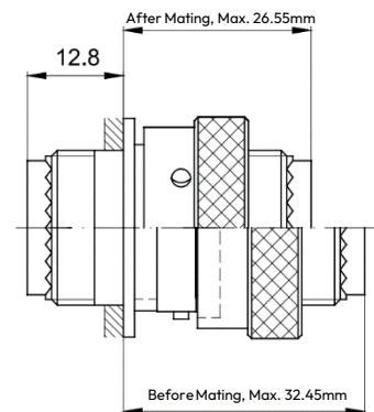
MS27513 Receptacle / MS27473 Plug
