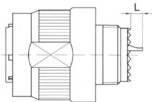
D38999/26 Receptacle
