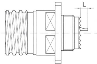
D38999/26 Receptacle
