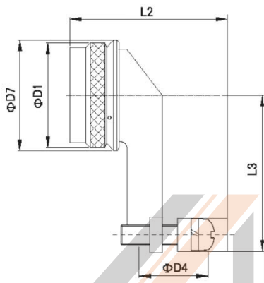
M85049/47 - (HC Type) Angled Cable Clamp
