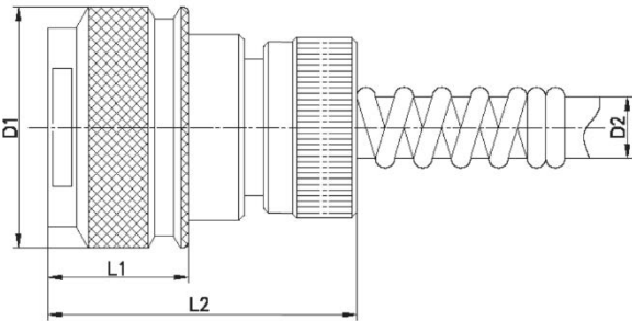
M85049/06 - Spring-loaded cable protection type backshell
