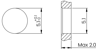
Recommended Panel cut-out
