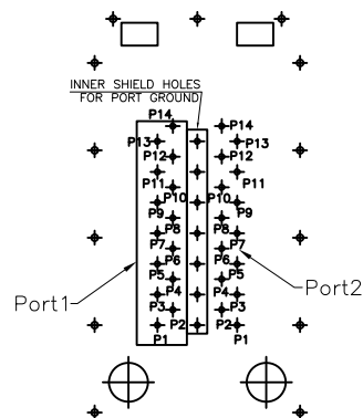
Pin OUT Information Component Side View
